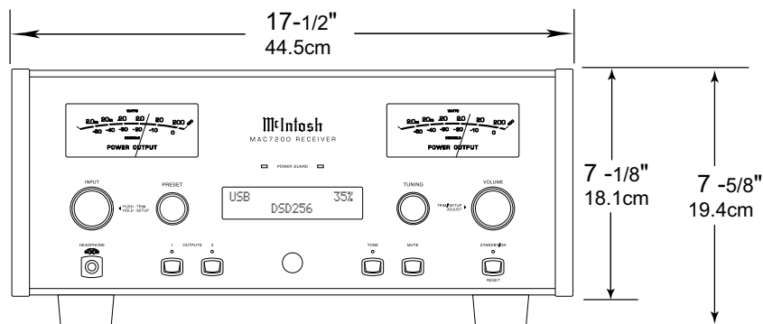
Front View of the MAC7200
