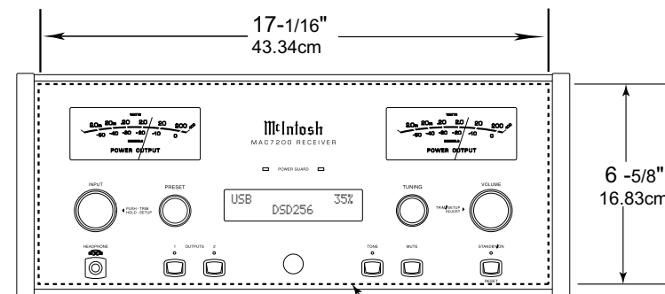
MAC7200 Front Panel Custom Cabinet Cutout
