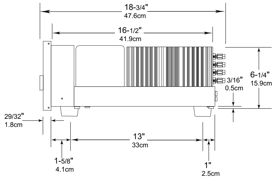
Side View of the MAC7200
